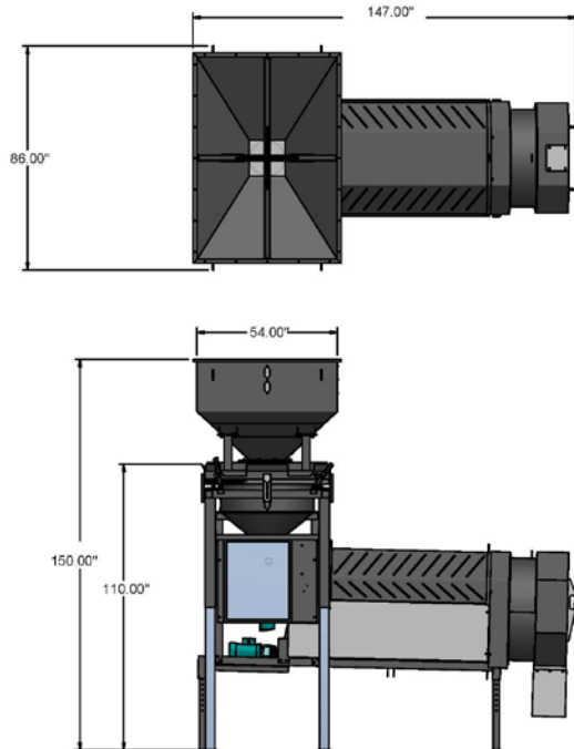
LIW MOUNTED OVER TREATER
