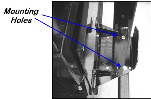
Top View of Flow Meter Bracket on Tower Support Bar
